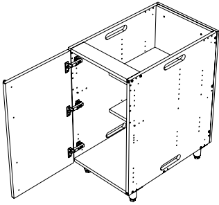
SINGLE DOOR BASE with 2 shelves 18"W x 34.5"H x 27"D B1827FH-xxx
