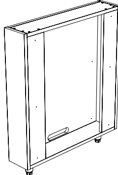
REFRIGERATOR SUPPORT END 6"W x 34.5"H x 27"D RSE0627-xx
