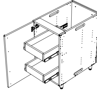
SINGLE DOOR BASE with 2 rollout trays 18"W x 34.5"H x 27"D B1827FHLIB-2T-xxx
