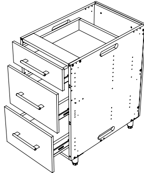
3-DRAWER BASE 18"W x 34.5"H x 27"D B3D1827-xxx
