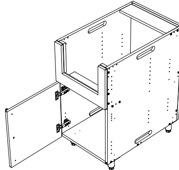
SIDE BURNER BASE 18"W x 34.5"H x 27"D GB1827-xxx
