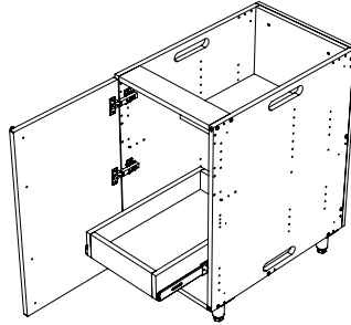
SINGLE DOOR BASE with 1 shelf & 1 rollout tray 18"W x 34.5"H x 27"D B1827FHLIB-1T-xxx
