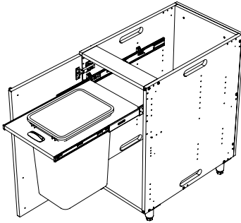
SINGLE DOOR BASE with trashcan pullout 18"W x 34.5"H x 27"D B1827FHLIB-TC-xxx
