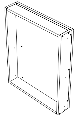
REFRIGERATOR BACKER BLOCK 15"W | 22"W | 24"W x 30"H x 5 1/8"D RBK1530-xxx | RBK2230-xx | RBK2430-xx
