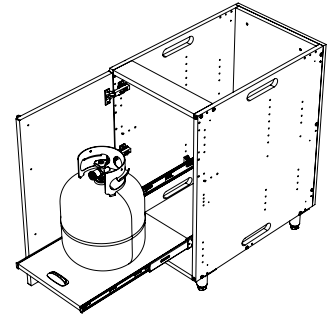
SINGLE DOOR BASE with propane tank pullout 18"W x 34.5"H x 27"D B1827FHLIB-PP-xxx
