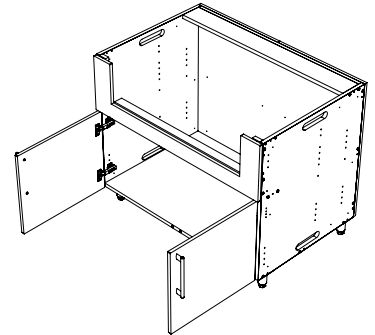
2 DOOR GRILL BASE 30"W | 42"W | 48"W x 34.5"H x 27"D GB3027-xxx | GB4227-xxx | GB4827-xxx
